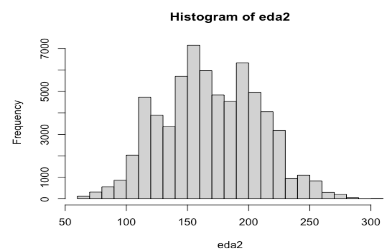
Fig 2. Histogram of Rainfall averages from days Jan-10, Dec-20 (days shown in x-axis)
